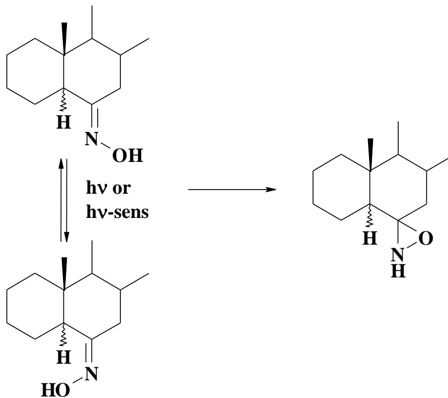
oxaaziridine
