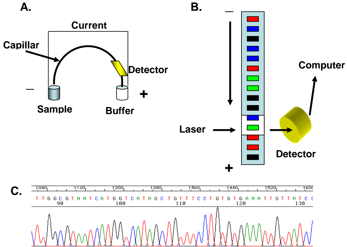
Figure 6. Schematic representation of a capillary-based DNA sequencing system. A. The basic set up of a capillary system. The sequencing reaction is placed in the sample holder, the electrophoresis buffer is held in the second holder, the capillary has been filled with polymer, and the electrophoresis current is applied through the capillary. B. False color representations of the resolving sequence fragments running past the optical window, being excited by the laser, the detector reading emission wavelengths and sending that information to the computer where the software has been trained for base calling. C. The final sequence electropherogram output.
